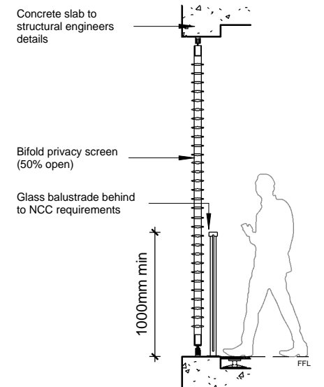
3. Screen Detail Scale 1 : 50
