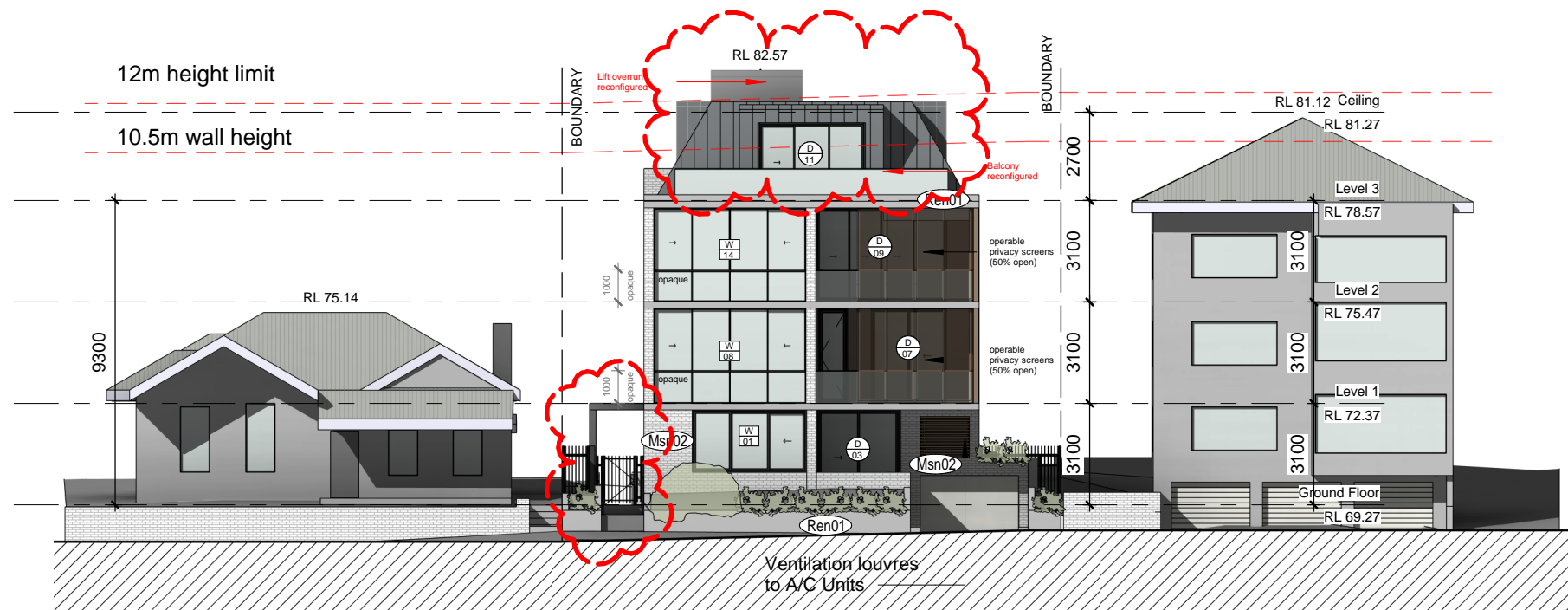
1. West Scale 1 : 200
